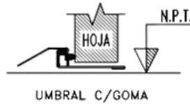
UMBRAL C/GOMA
